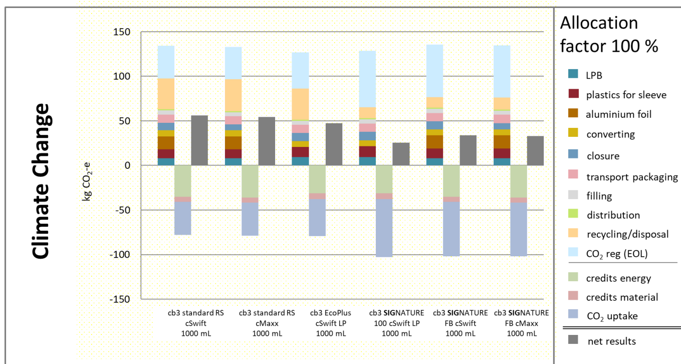
Figure 3-2: Climate Change results of scenario II Belgium, combiblocSlimline (cb3) beverage cartons with allocation factor 100%
