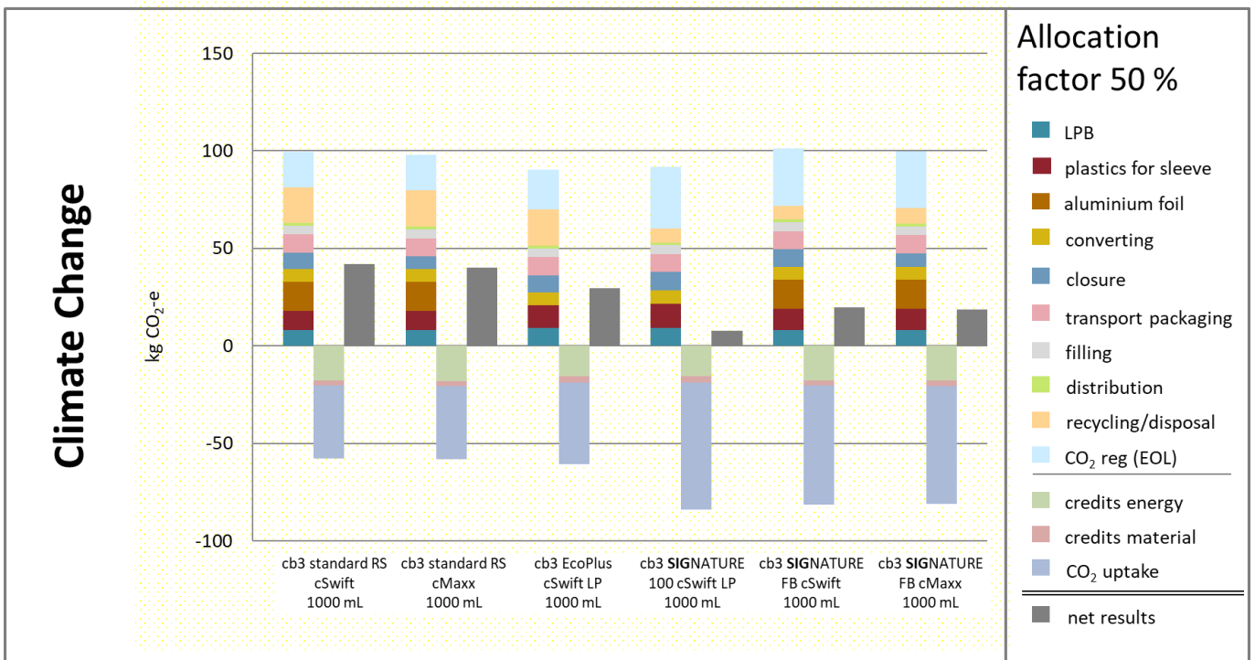
Figure 3-1: Climate Change results of scenario I Belgium, combiblocSlimline (cb3) beverage cartons with allocation factor 50%
