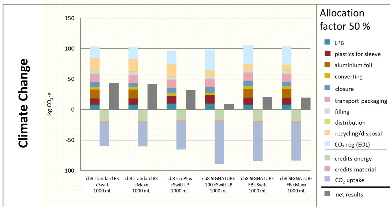
Figure 3-3: Climate Change results of scenario I Belgium, combiblocMidi (cb8) beverage cartons with allocation factor 50%
