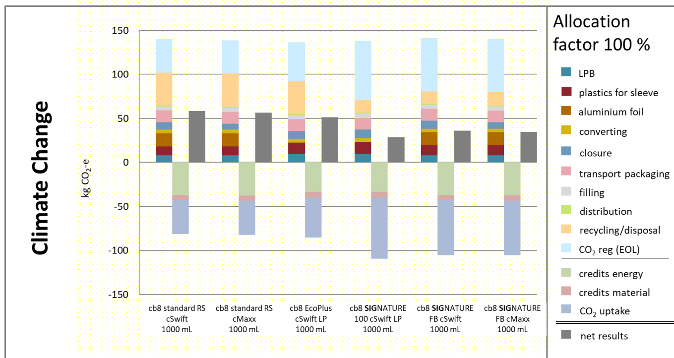
Figure 3-4: Climate Change results of scenario II Belgium, combiblocMidi (cb8) beverage cartons with allocation factor 100%
